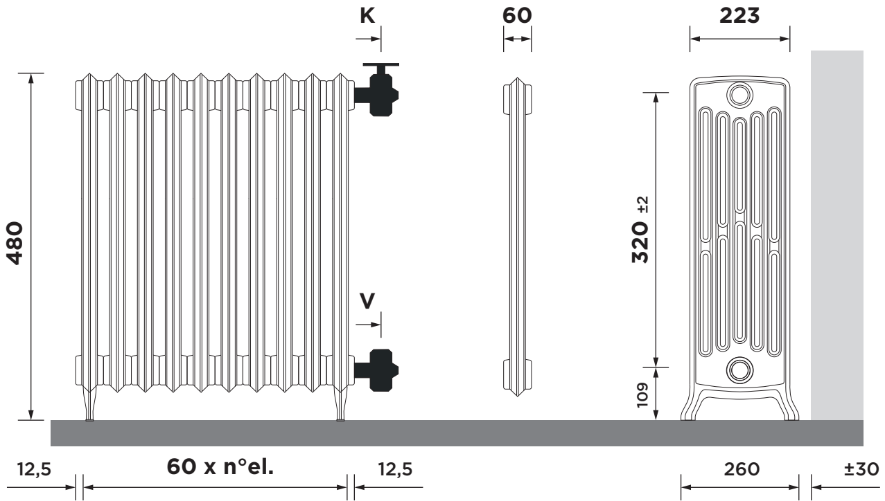
on the floor | bodenstehend | vloorstaand | na zemi | на полу/ногах BI6/480-F, all dimensions in mm ±2
