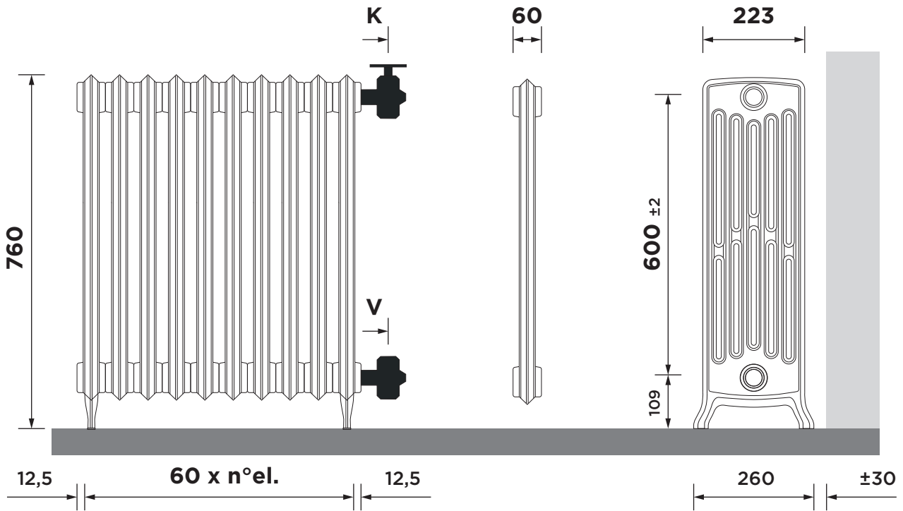
on the floor | bodenstehend | vloerstaand | na zemi | на полу/ногах BI6/760-F, all dimensions in mm ±2
